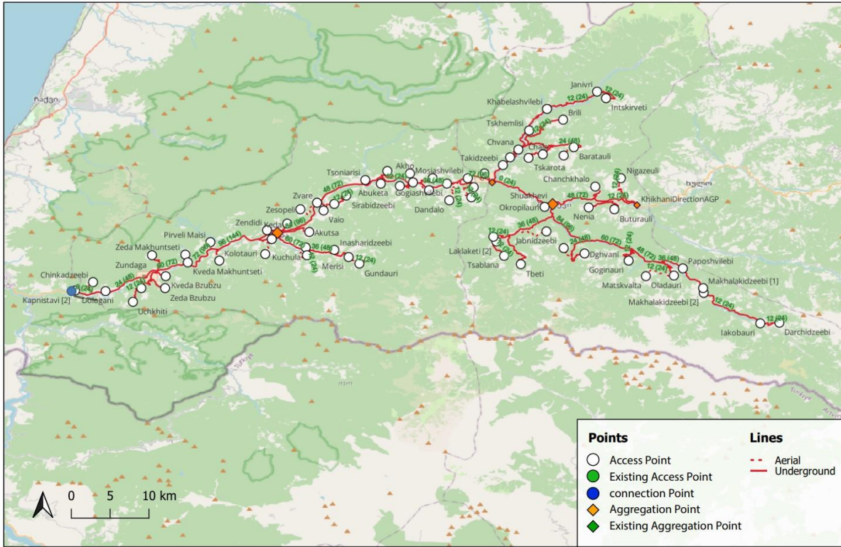
ANNEX 2, Fiber-optic recommended route
